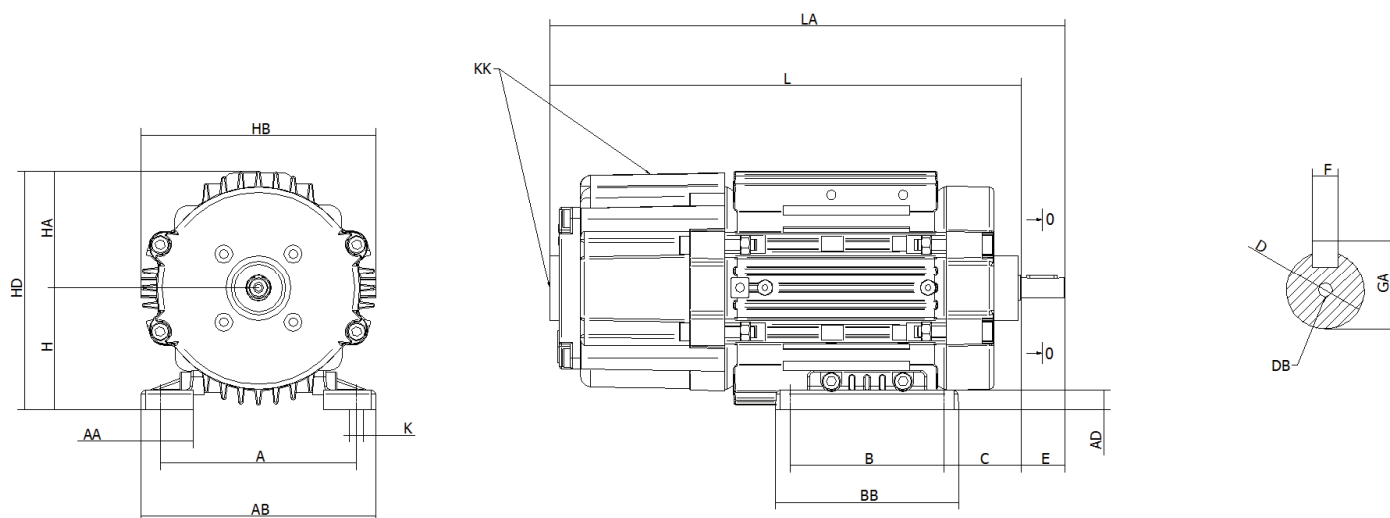
Mounting B3
